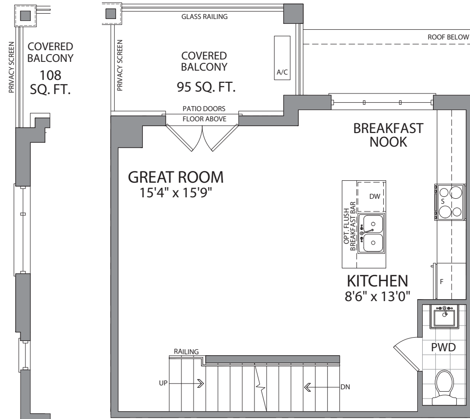
SECOND FLOOR EXTERIOR END UNIT
