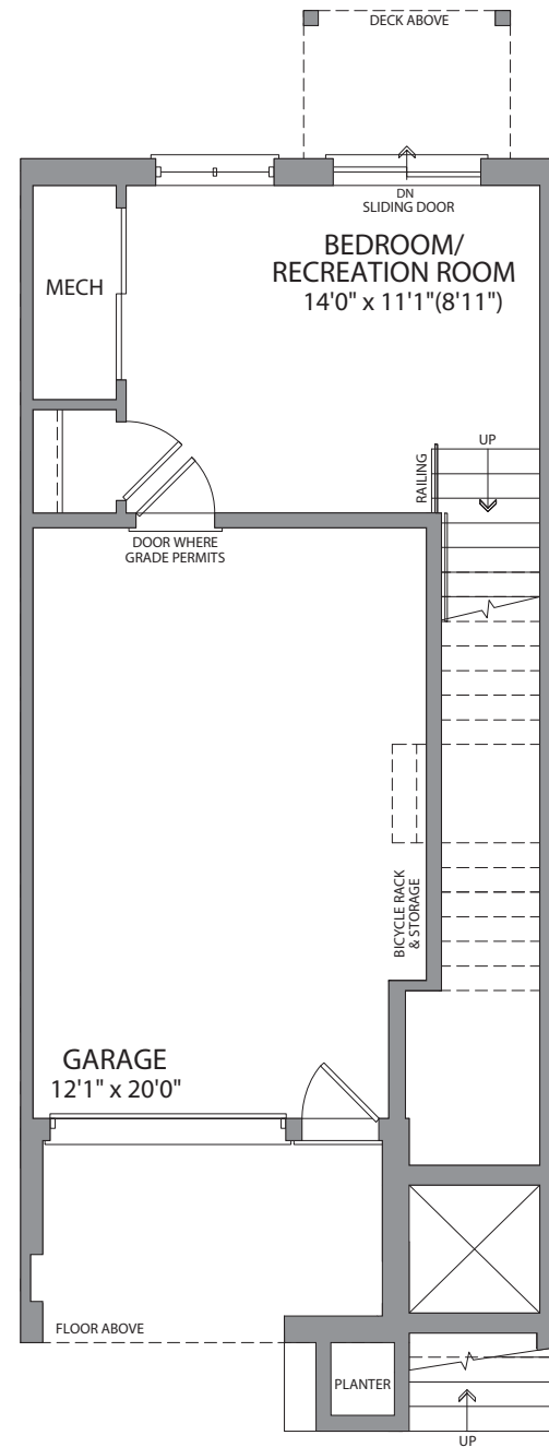
GROUND FLOOR
