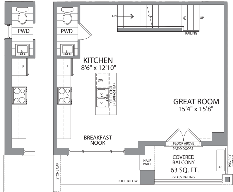
SECOND FLOOR EXTERIOR END UNIT
